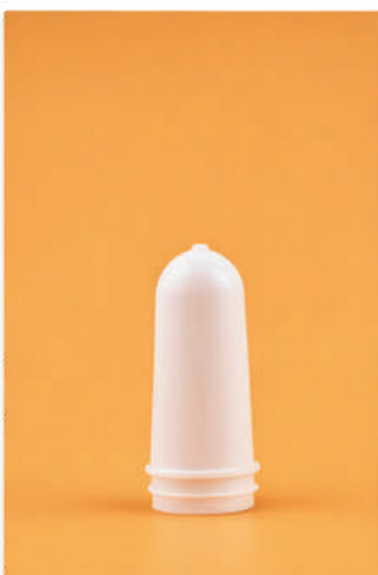
PREFORM D42 Weight | 17.5 Gram Height | 63.2 mm
