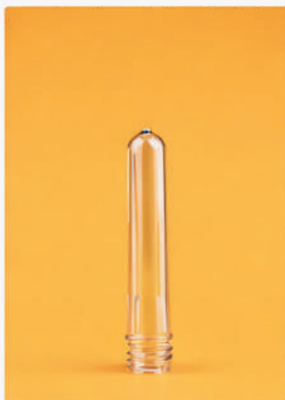
PREFORM D18 Weight | 12.5 Gram Height | 94 mm
