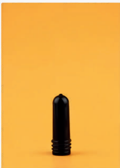
PREFORM D18 Weight | 5 Gram Height | 53.3 mm
