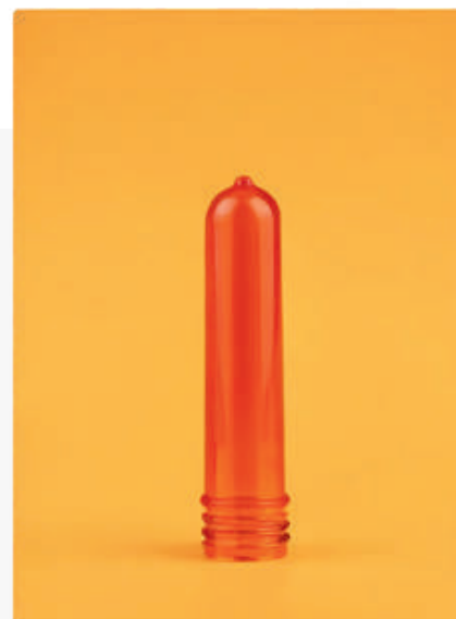
PREFORM D24 Weight | 23 Gram Height | 104.6 mm
